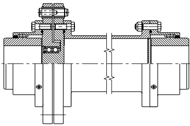
Type MTBLX Spacer shear pin coupling
