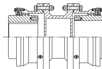
Type MTAD for high misalignment
