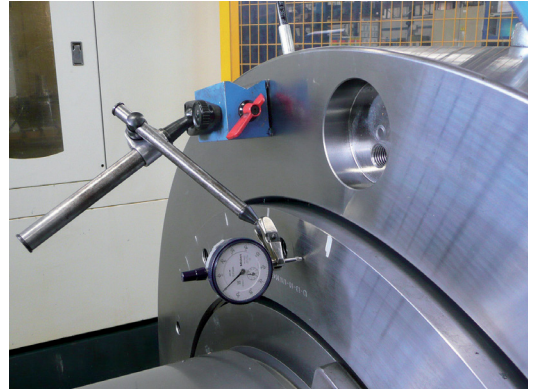
Drive-up measurement on JHC-HS-750
