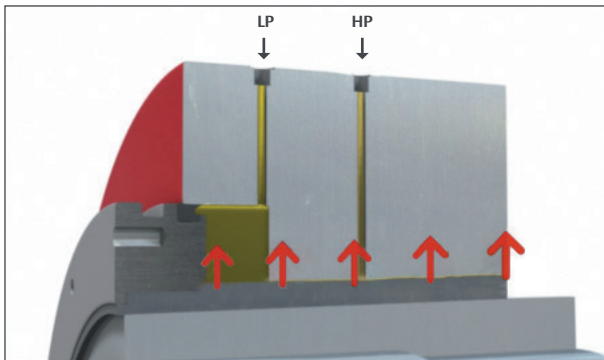
3 Once the oil layer has fully separated both surfaces, low pressure (LP) oil is injected into the chamber in order to exert the necessary axial force for driving up the outer sleeve. This operation will continue until a given axial "drive-up" value is reached.
