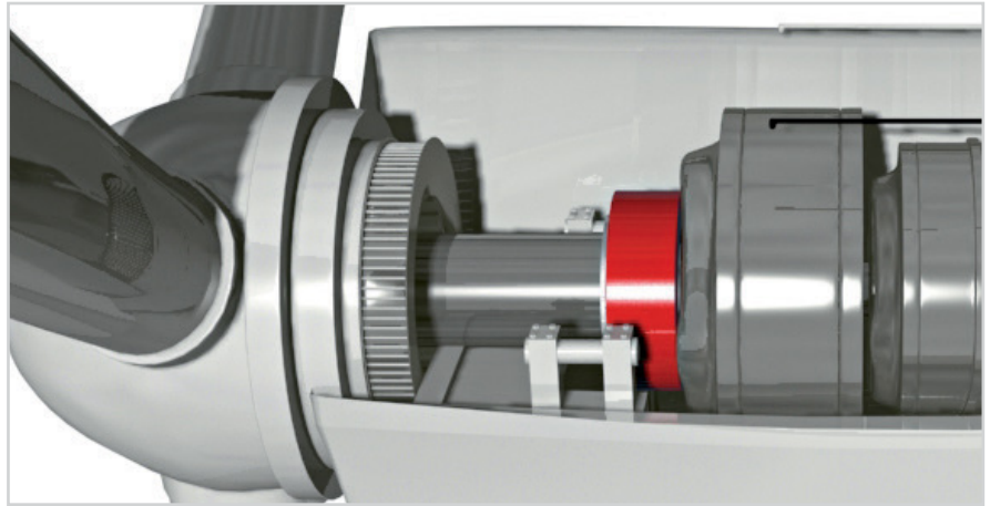
Jaure JHC-HS on a 3Mw wind turbine LSS
