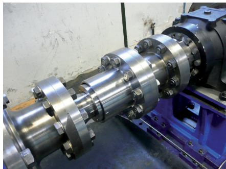
In house fatigue testing JHC-HF-F-100
