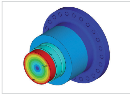
FEA of JHC hydraulic couplings
