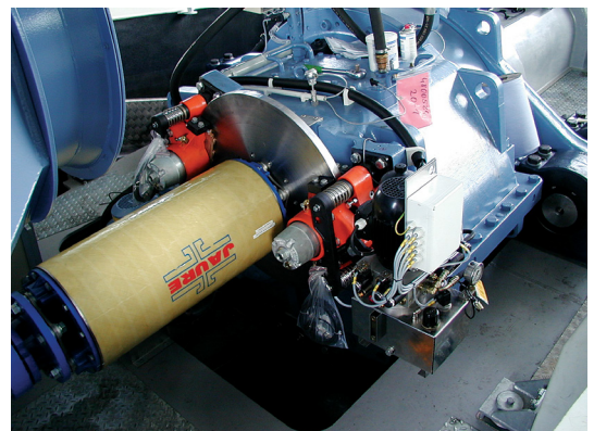
LAMIDISC coupling in combination with glass fiber shaft for electrical insulation
