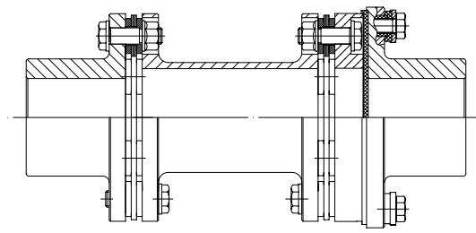
Type SXAE. With electrical insulation.
