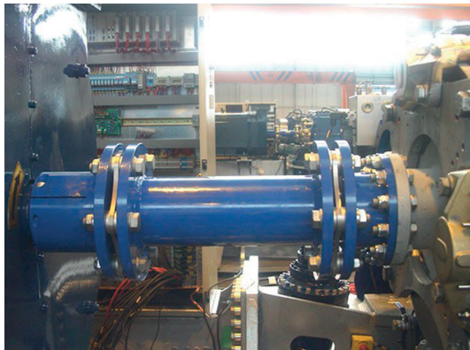
LAMIDISC™ coupling SXPR with adaptor flange
