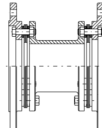
Type SXP. With flange adaptors.
