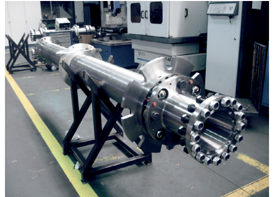
LAMIDISC coupling 380-8 with locking device and bulkhead seal for marine drive
