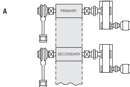
Figure 5 — Dual motor, dual backstop, dual pulley arrangement –
