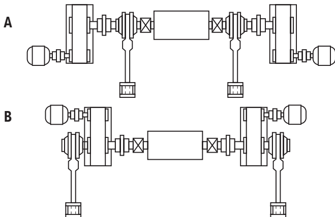
Figure 3 — Tandem motor, tandem backstop, single pulley arrangements –
