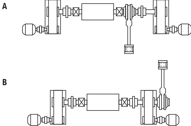
Figure 2 — Tandem motor, single backstop arrangements –
