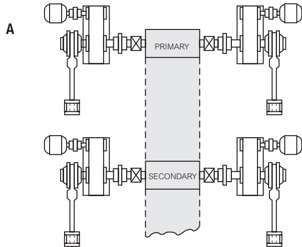
Figure 4 — Tandem motor, tandem backstop, dual pulley arrangement –
